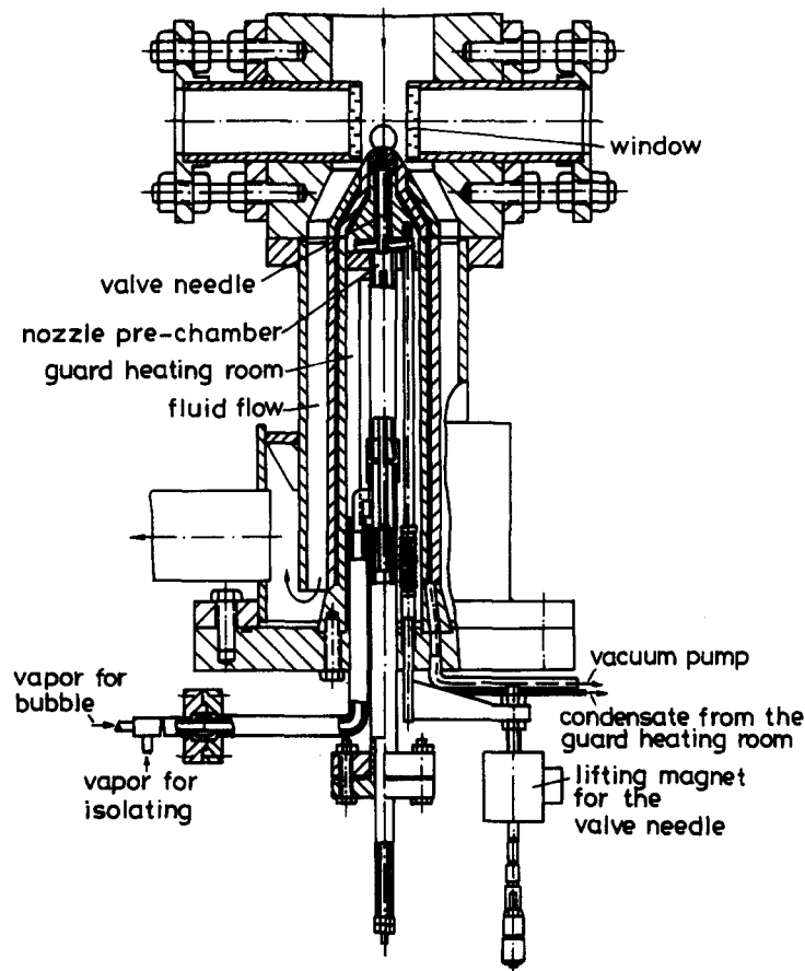
Figure 1. Test section.
