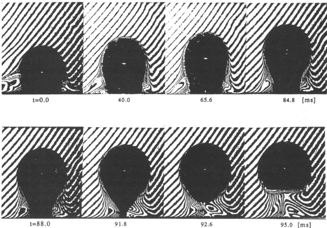
Figure 5. Interferograms of a condensing propanol bubble ( p = 2 bar, \Delta T = 7.6 K, Ja = 7.1 ).
