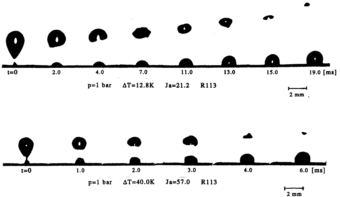
Figure 9. Temporal decrease in the bubble volume.
